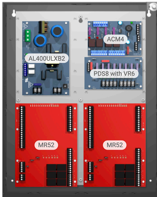
T1MK14S 4-Door Access System with Power
