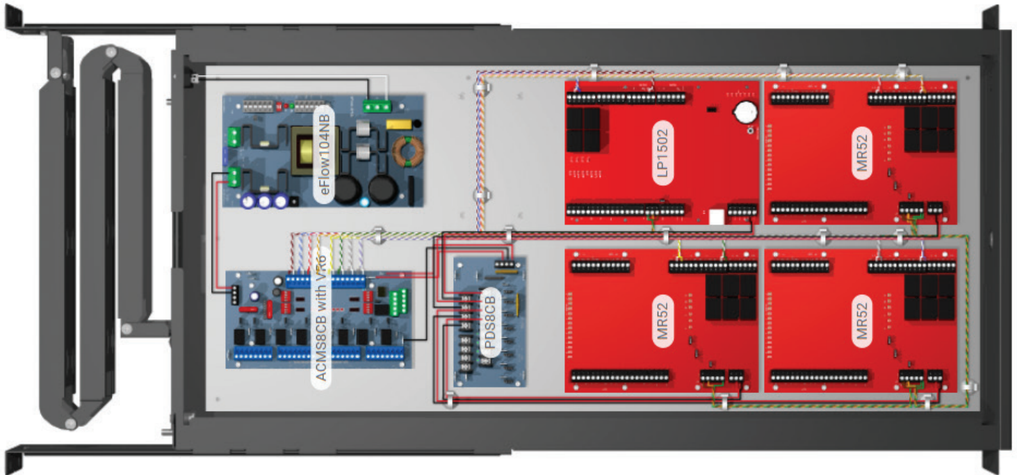
T1RM7CK1D 8-Door Rack Access System with Power
