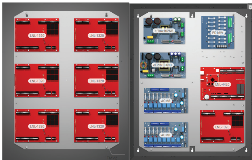
T2MK75F16 16-Door Access System with Power
